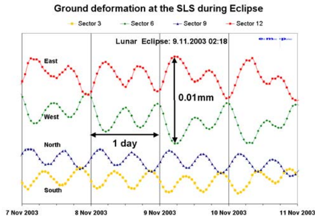
Figure10: A four day period of the year 2003 with a time resolution of 1 hour. The influence of the earth tides with 2 periods a day is clearly visible. Note the high amplitude difference between east and west during the eclipse of the moon.
